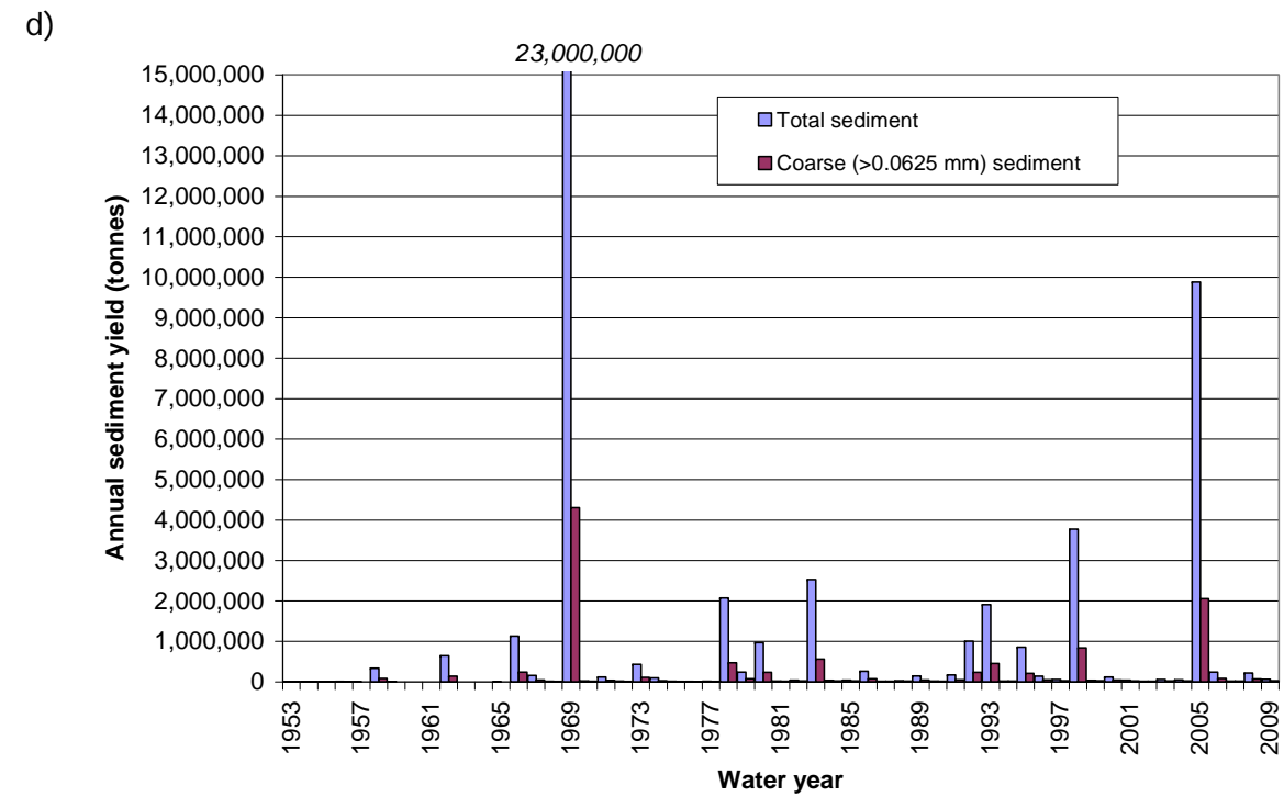
Figure 4-1d. Calculated total sediment yield (suspended load + bedload) and coarse (>0.0625 mm) sediment yield for the USCR at the County line between 1953 and 2009 (USGS 1118500 and 11109000).
