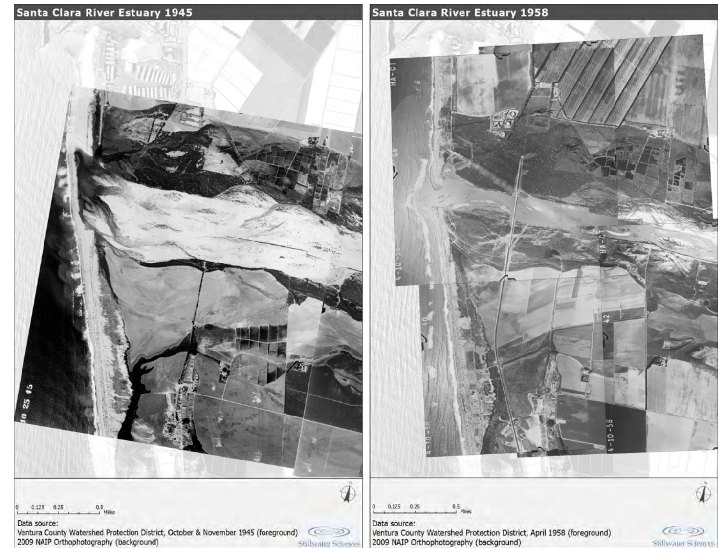
Figure 5-9. SCRE and surrounding floodplain (1945 and 1958).
